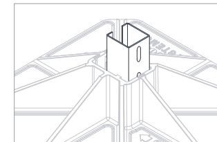
40 x 38 x 1.9mm Euro Strut
